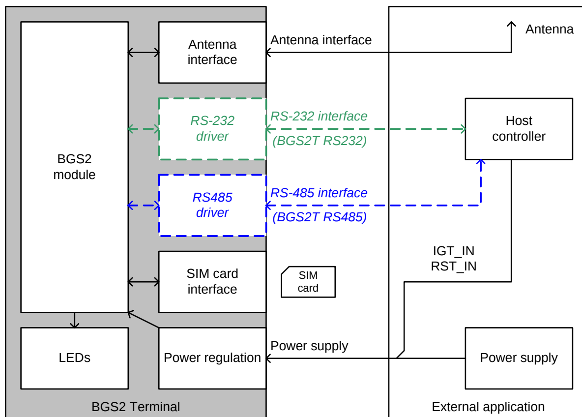
Figure 3: Block diagram
