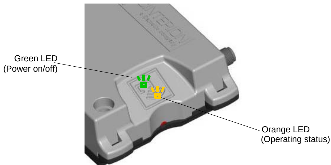
Figure 9: Status LED
