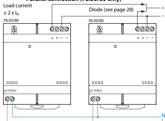
Parallel connection (78.50/60 only)
