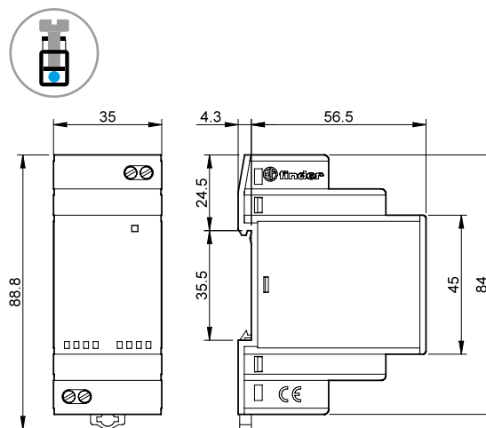
Type 78.25...1202/2482 Box clamp
