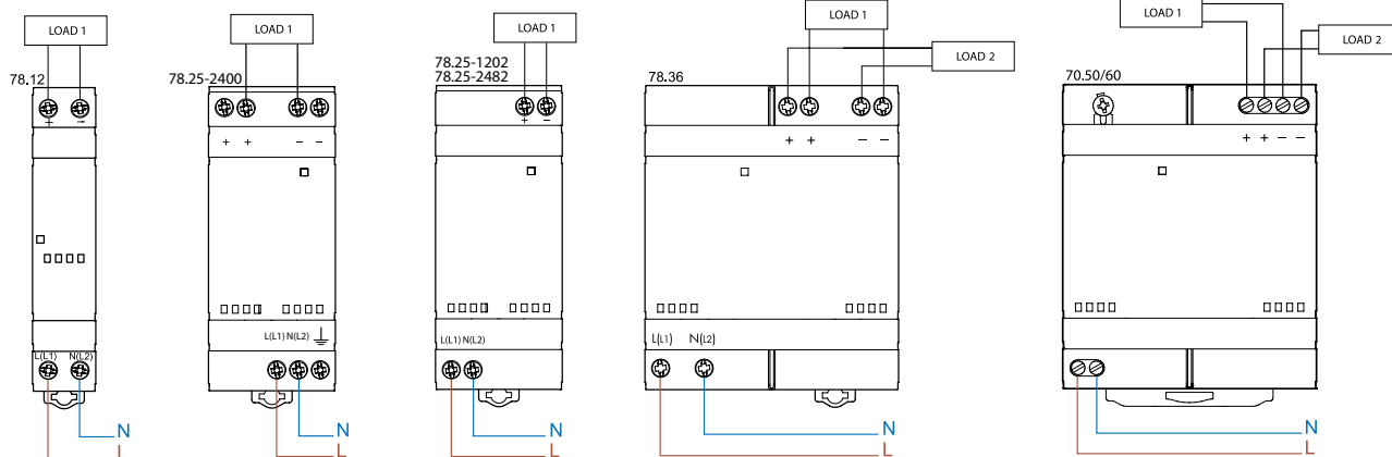
Dual polarity connection
