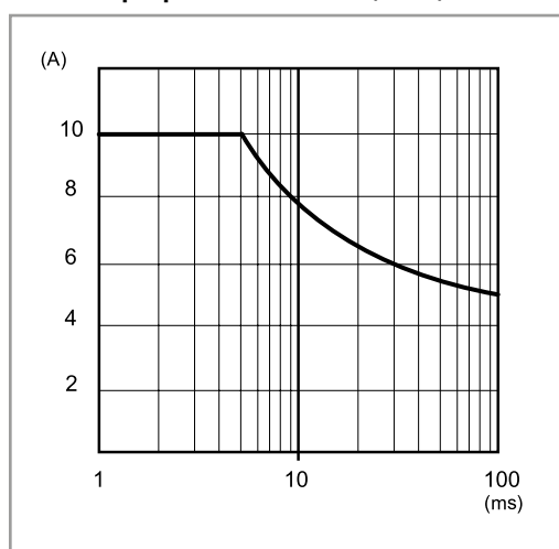
P78-7 Output peak current v time (78.1B)
