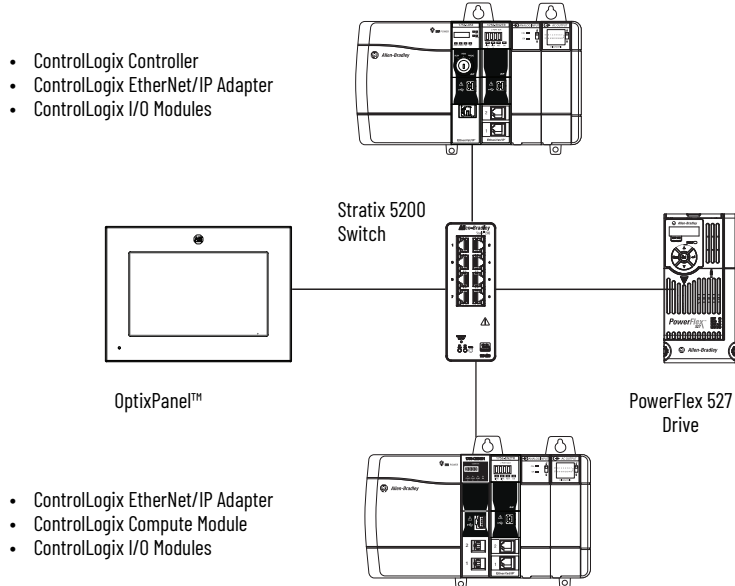
Compute Module Communication Over EtherNet/IP Network and Controller Chassis Backplane
