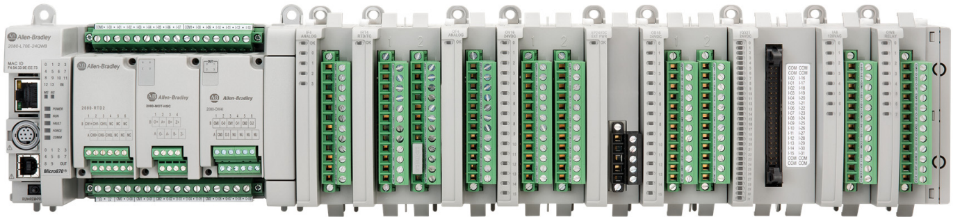
A Micro870 controller with plug-in modules, eight expansion I/O modules, and an expansion I/O power supply attached
